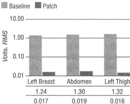
Figure 7-1. The graph shows the huge difference in environmental electric field potential measured on the body at three sites—at baseline, that is, before grounding, and during grounding.
